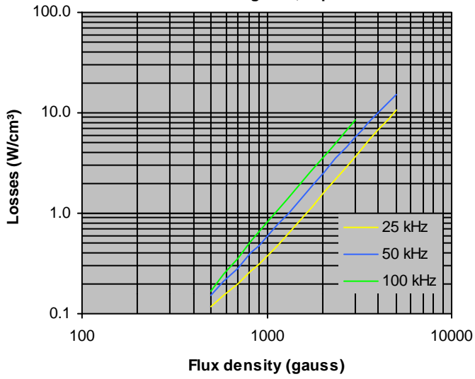
Power Loss Density vs Flux Density 83 grade, 60 \mu i
