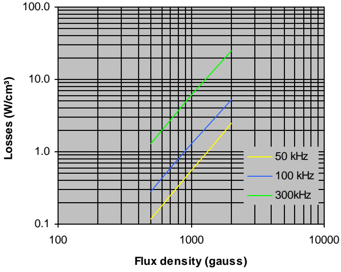
Power Loss Density vs Flux Density 85 grade, 125 \mu i
