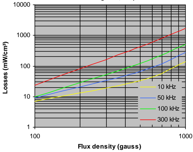
Power Loss Density vs Flux Density 96 grade, 147 \mu i
